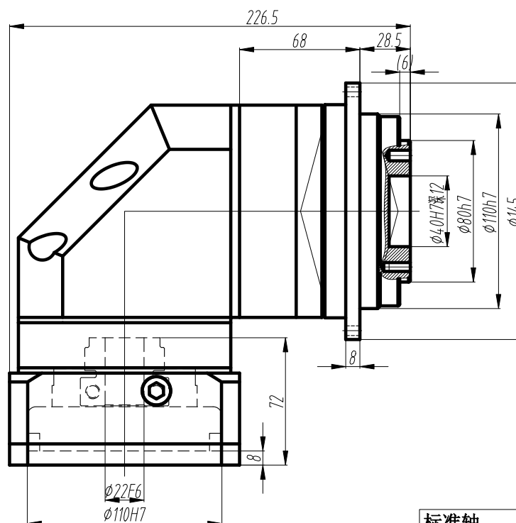
Standard output shaft
